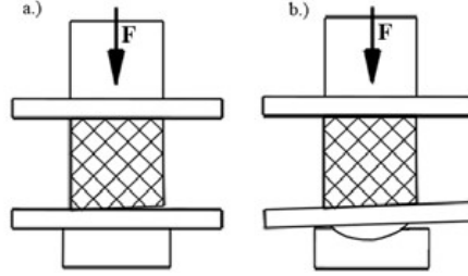
Figure 1 Measurement setup: a) Parallel plate, b) Self-aligning compression plate
